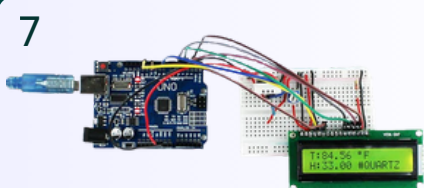
Temperature & Humidity Monitor System
