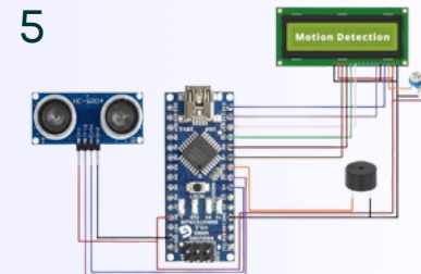
Motion Detection System
