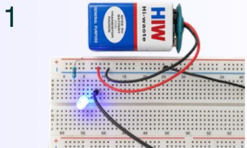
LED Circuit - using Battery & Breadboard
